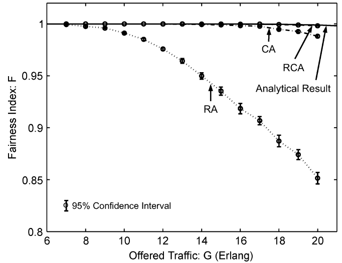
Fig. 10. Fairness index, Case II .
